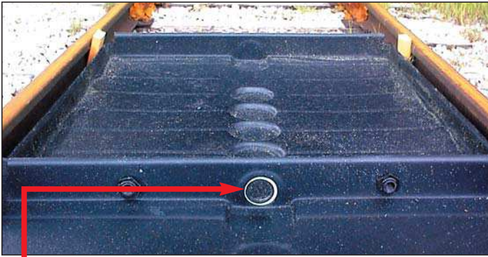
Large, 76 mm diameter flow-through channels allow spills to quickly travel from one pan to the next. Channels are located at the low point in each Center and Side TrackPan.
