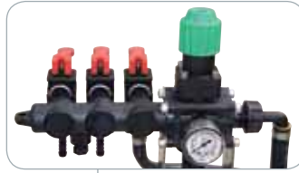
Pressure regulator, gauge & manifold for easy boom spray control
