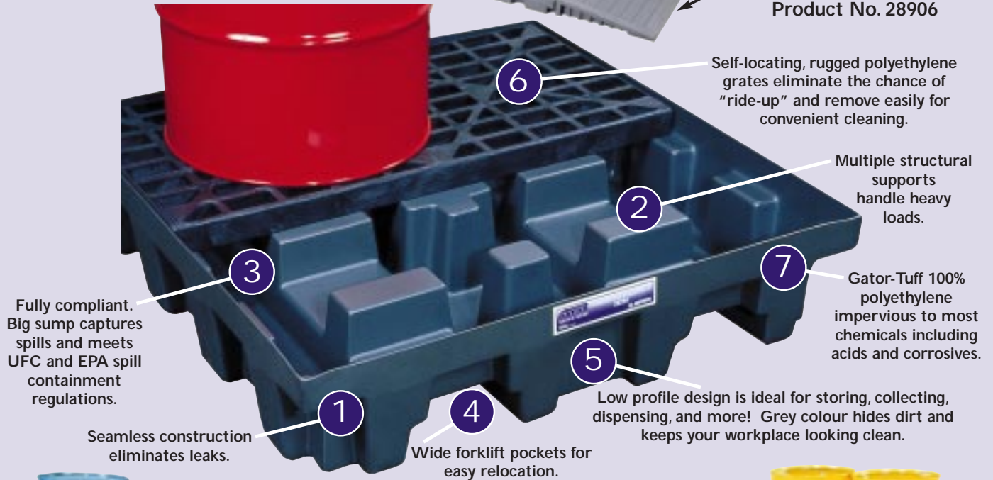
4-Drum Square Pallet Product No. 28254
