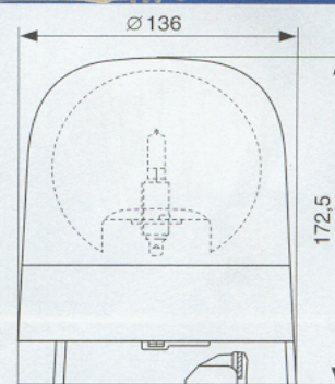
Form D as per ISO 4148
